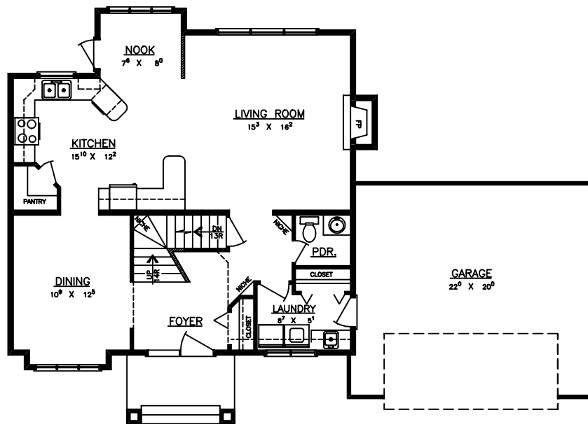
MAIN FLOOR AREA = 966 S.F.
