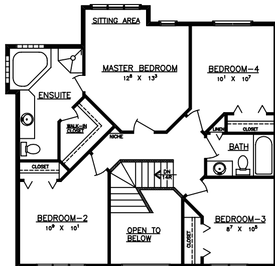
SECOND FLOOR AREA = 855 S.F.
